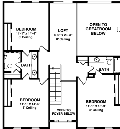
UPPER LEVEL FLOOR PLAN 1007 sq ft
